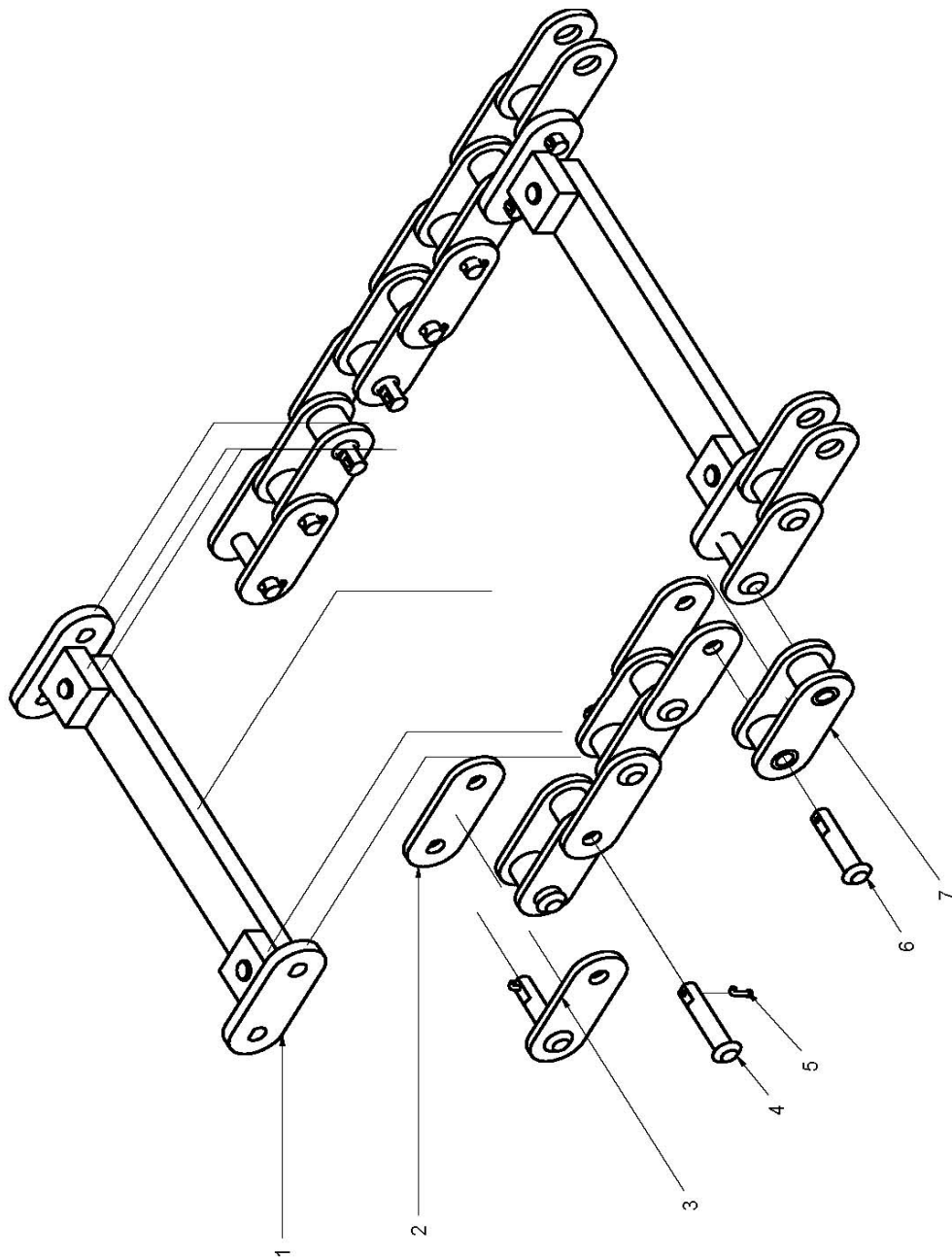
Conveyor Chain Complete
