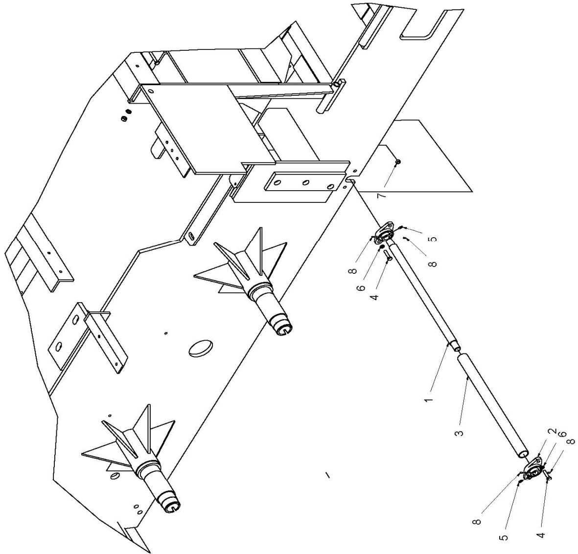
Conveyor Chain Support Assembly
