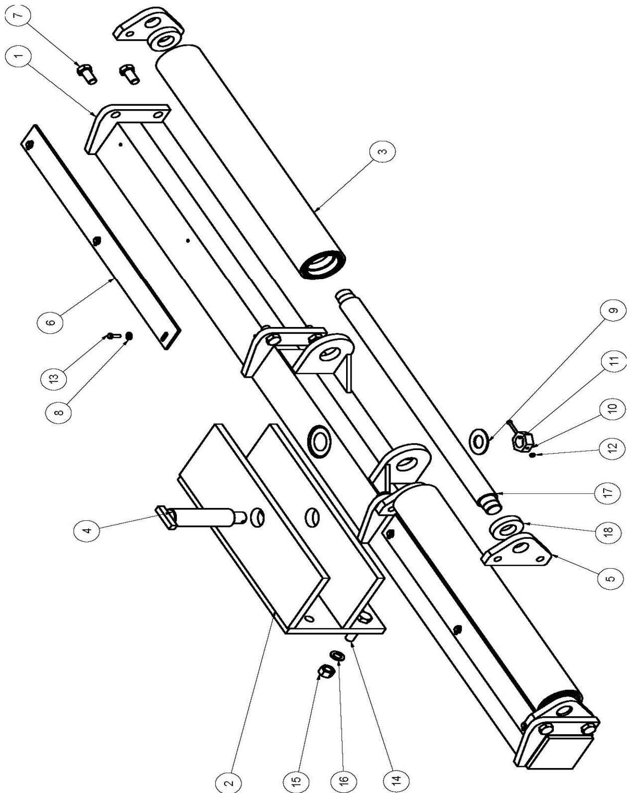
PUSH ROLLER ASSEMBLY
