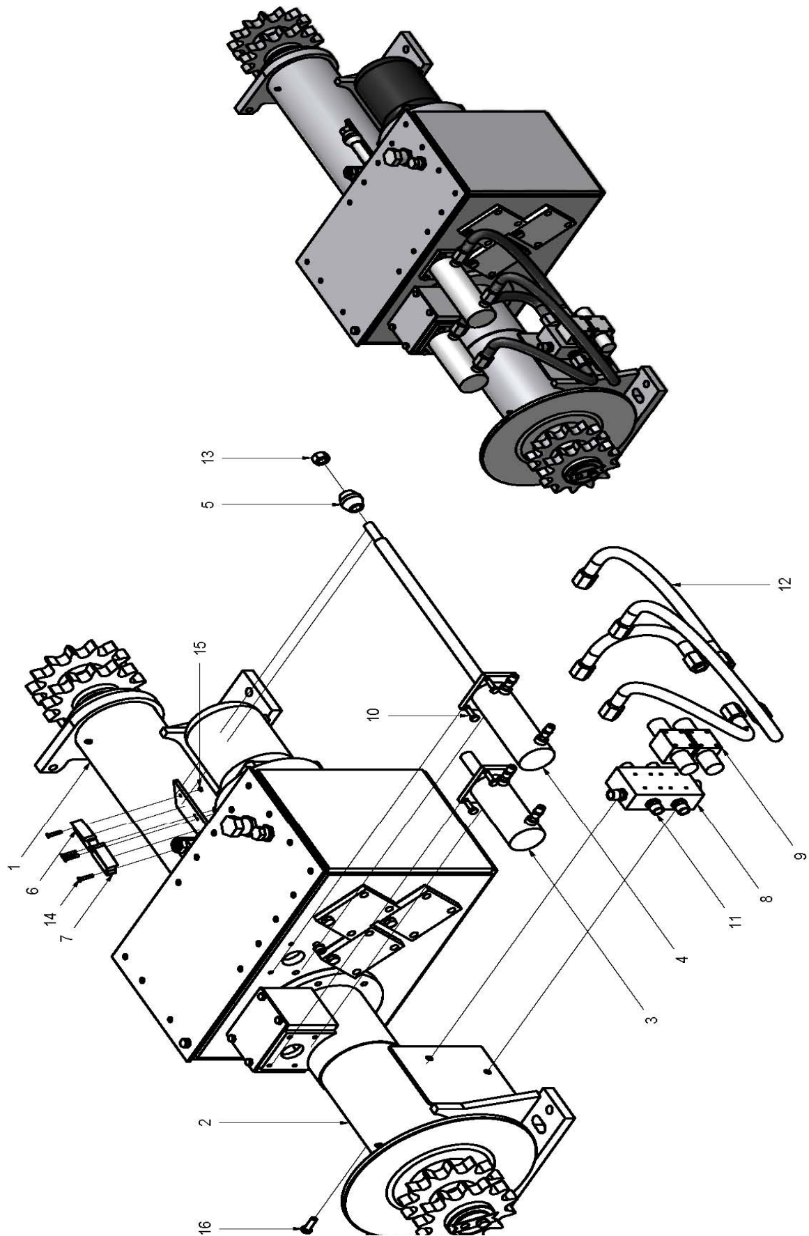
Drive Axle Electro Hydro Control
